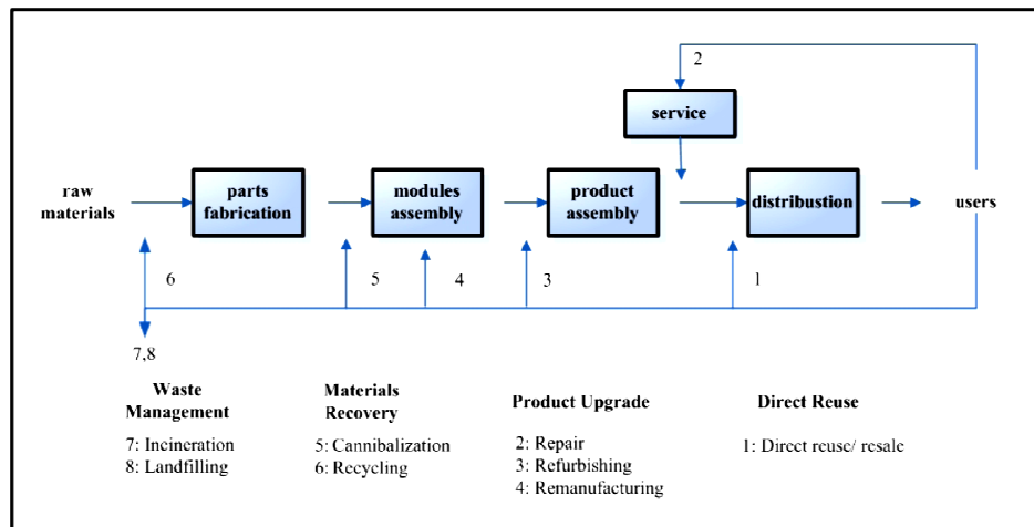
Figure 1. Product regeneration path diagram of closed-loop supply chain [9]
