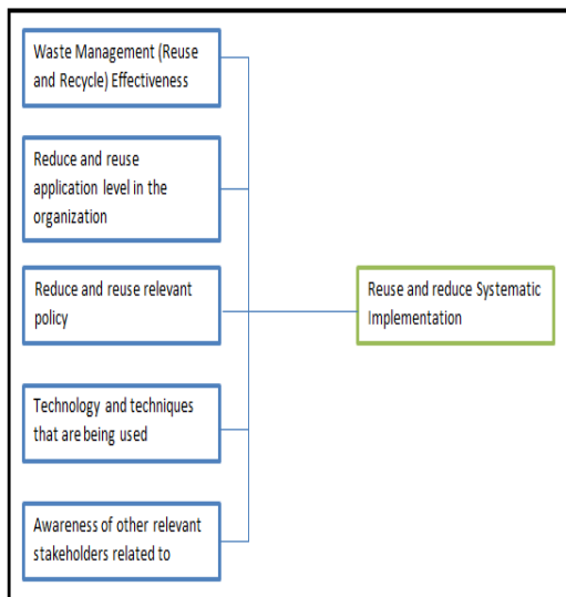
Figure 1. Research Framework
