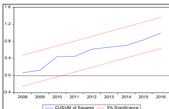
Figure 4. Cumulative Sum of of Square of Recursive Residuals
