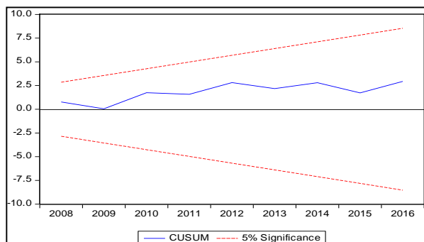
Figure 3. Cumulative Sum of Recursive Residuals (CUSUM)
