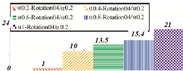
Figure 18- Rotation ratio of 4th story of 6-story structures to 4th story of 0.2\alpha structures under additional load in the Y direction in the plastic range
