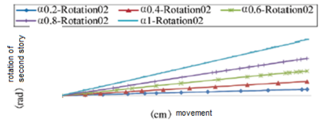
Figure 19- Class 2 diaphragm rotation 2-story structures under the effect of additional load in the X direction
