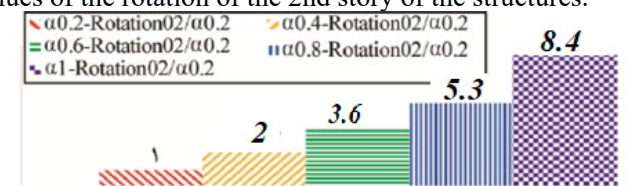
Figure 20- Rotation ratio of 2nd story of 2-story structures to 2nd story of 0.2\alpha structure under additional load in the X direction in the elastic range
