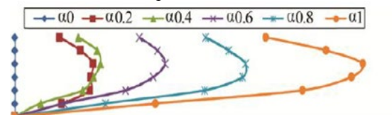
Figure 29- Rotation of the stories of 6-story structures under the Tabas earthquake record in the Y direction
