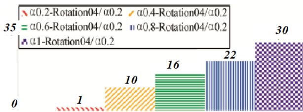
Figure 17- Rotation ratio of 4th story of 6-story structures to 4th story of 0.2\alpha structures under additional load in Y direction in the elastic range
